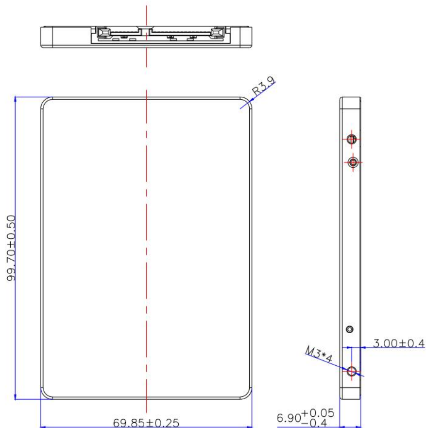
Figure 1: 2.5" SATA-III SSD Physical Dimension
