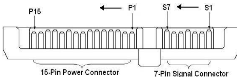
Figure 2: 7+15 Serial ATA port Interface Description
